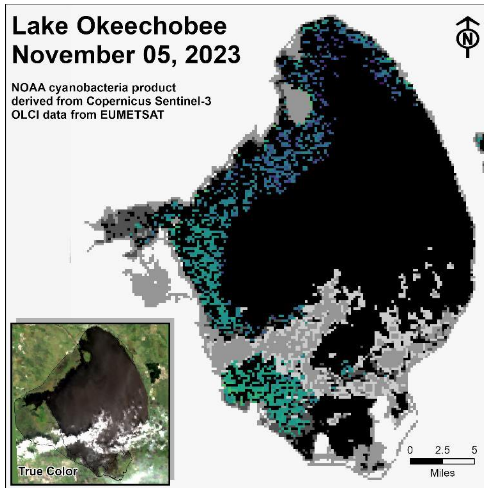
Figure LO-6. Cyanobacteria bloom index level on November 05, 2023, based on NOAA's harmful algal bloom monitoring system. Gray color indicates cloud cover.
