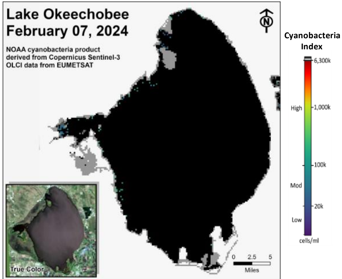
Figure LO-6. Cyanobacteria bloom index level on February 07, 2024, based on NOAA's harmful algal bloom monitoring system. Gray color indicates cloud cover.
