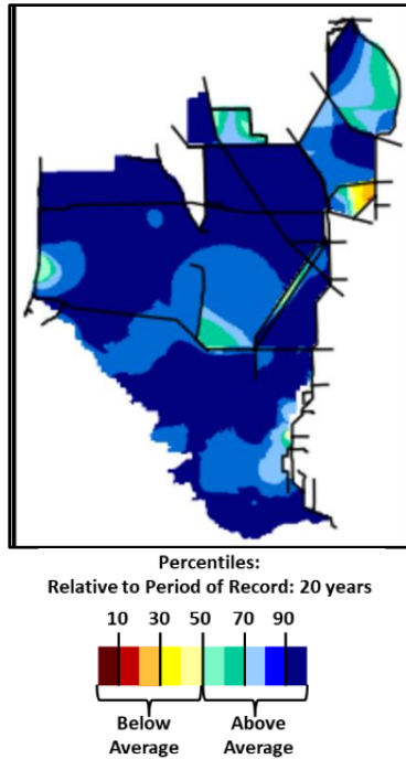
Figure EV-7. Present water depths (2/11/2024) compared to the day of year average over the previous 20 years.
