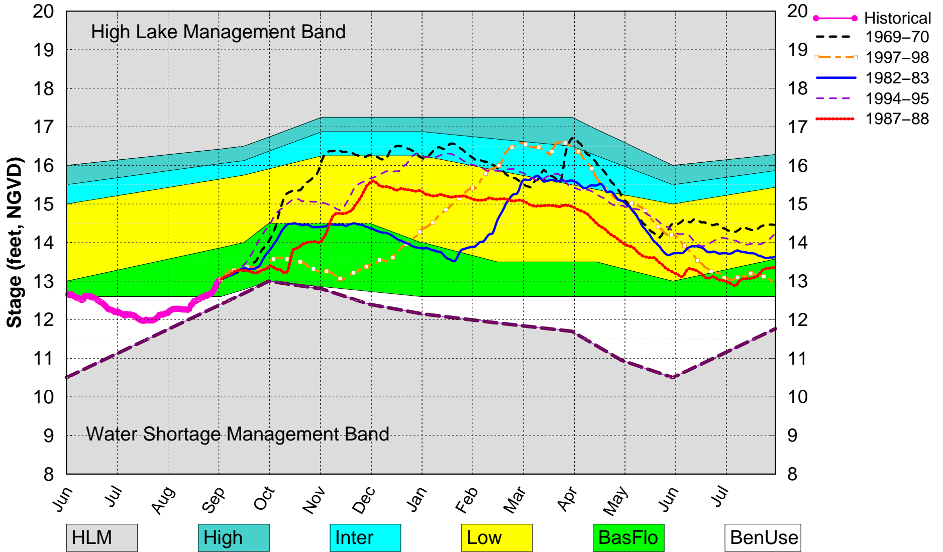
Wet Years Plot PA_SEP15DPA
