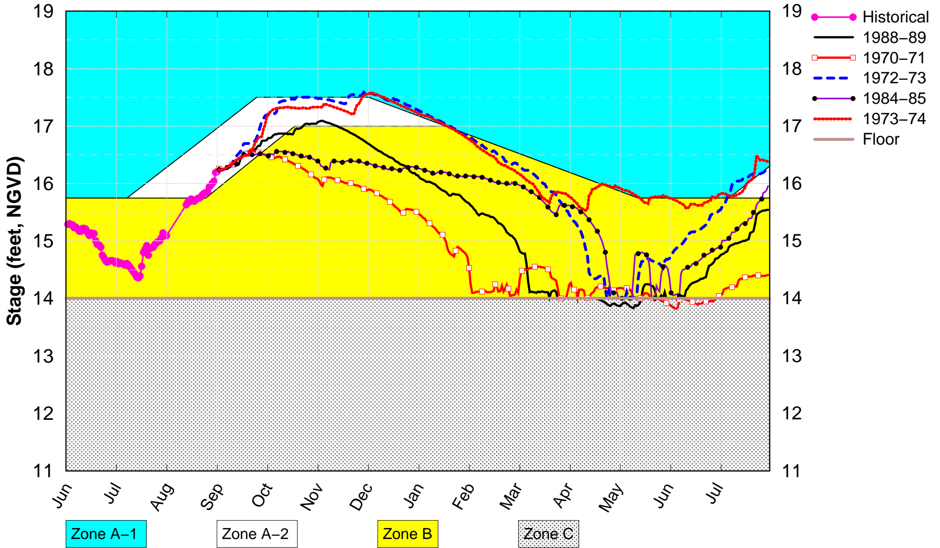
PA_SEP15DPA Dry Years Plot
