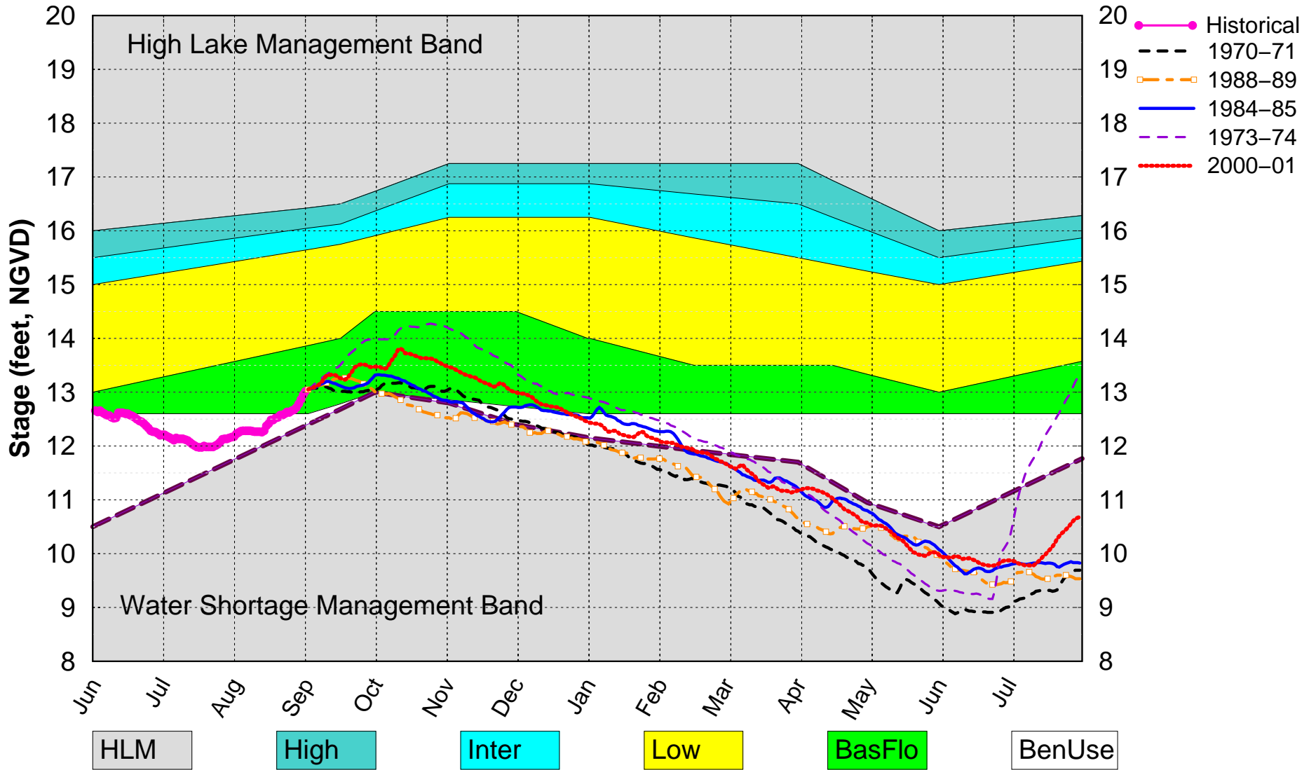
Dry Years Plot PA_SEP15DPA
