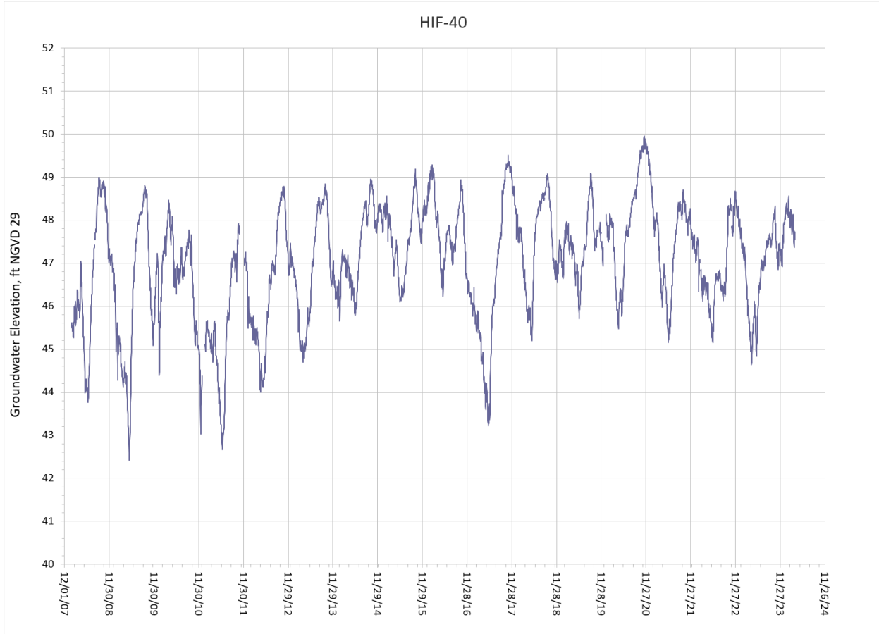
Figure 6-10. Groundwater elevations in Upper Floridan aquifer monitor well HIF-40, located at the C-41/C-41A Canal juncture in Highlands County.
