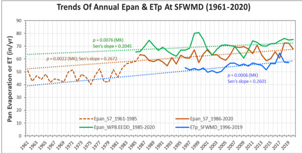
Figure 6-22. Trend of annual pan evaporation (Epan) and potential evapotranspiration (ETp) across the SFWMD, 1961 to 2020 (Cortez et al. 2022).
