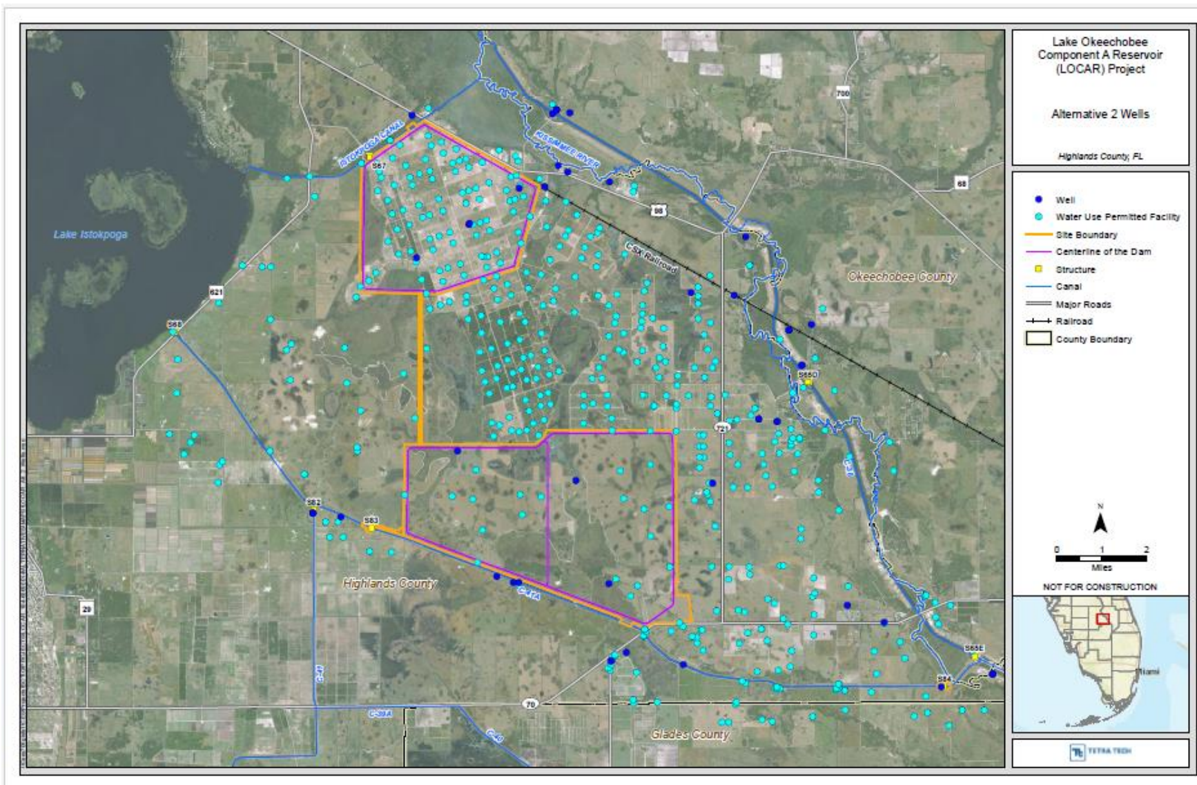
Figure E-12. Alternative 2, water supply wells and permitted use facilities.
