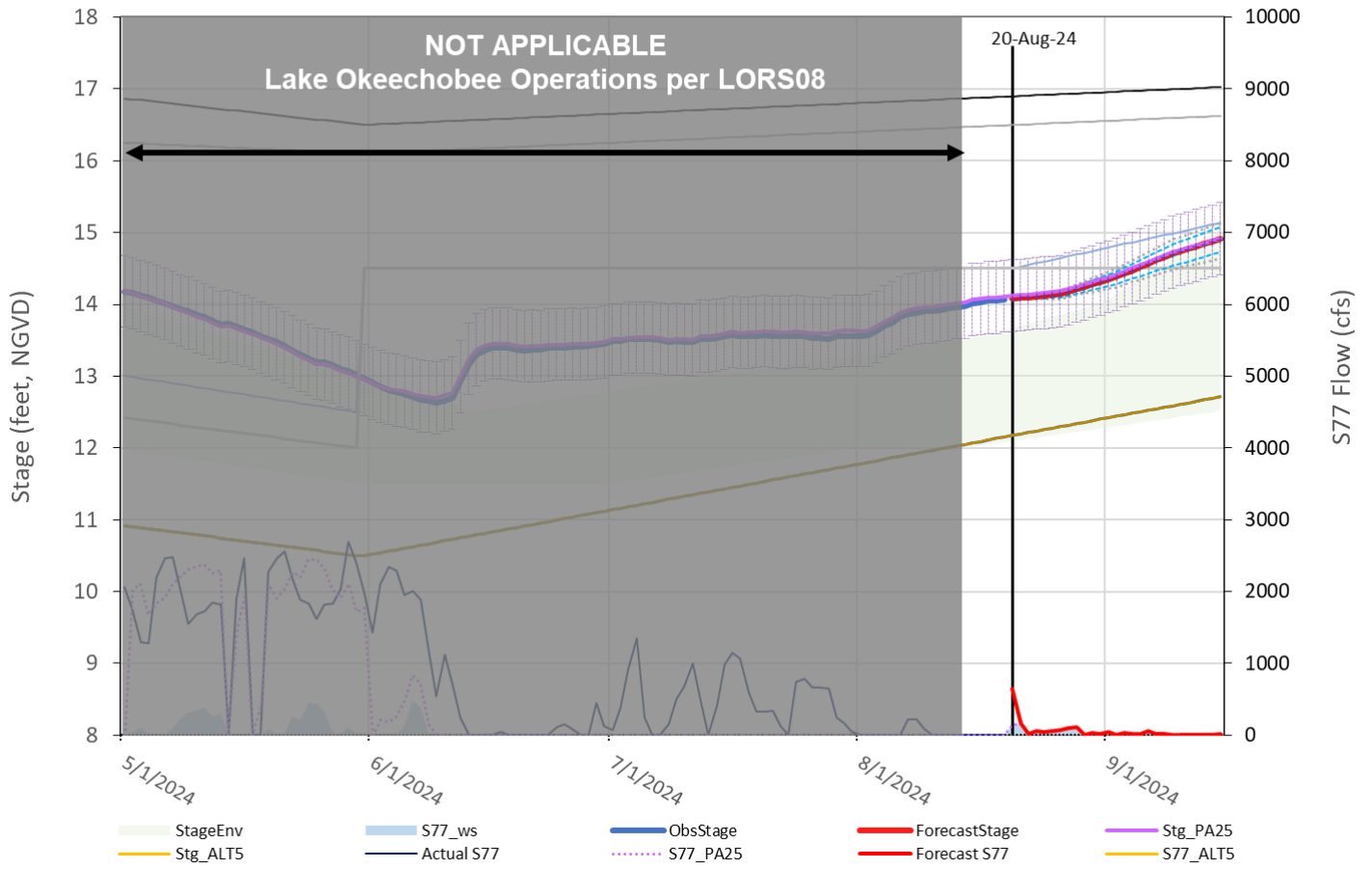
(b) LAT forecasted Lake Okeechobee stages and S-77 flows with 1200 cfs flow target at S-79
