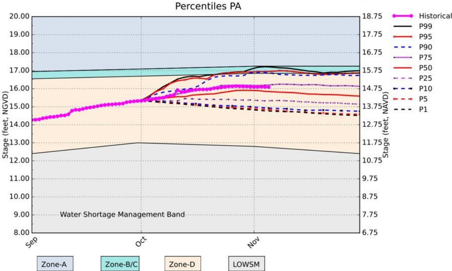
Lake Okeechobee October 2024 Conditional Position Analysis (PrefSce)
