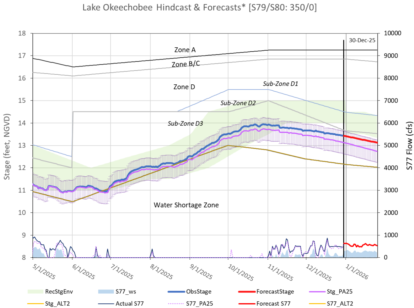
LAT-forecasted Lake Okeechobee stage and S-77 flows with 350 cfs target at S-79 and 0 cfs at S-80.
