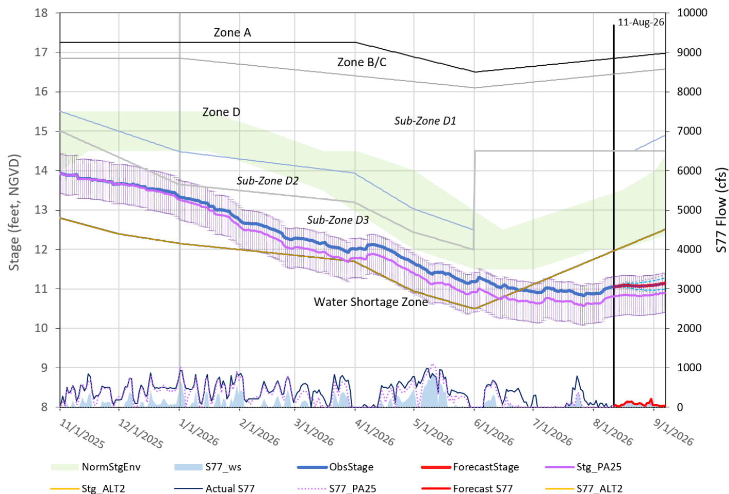
LAT-forecasted Lake Okeechobee stage and S-77 flows with 350 cfs target at S-79 and 0 cfs at S-80.
