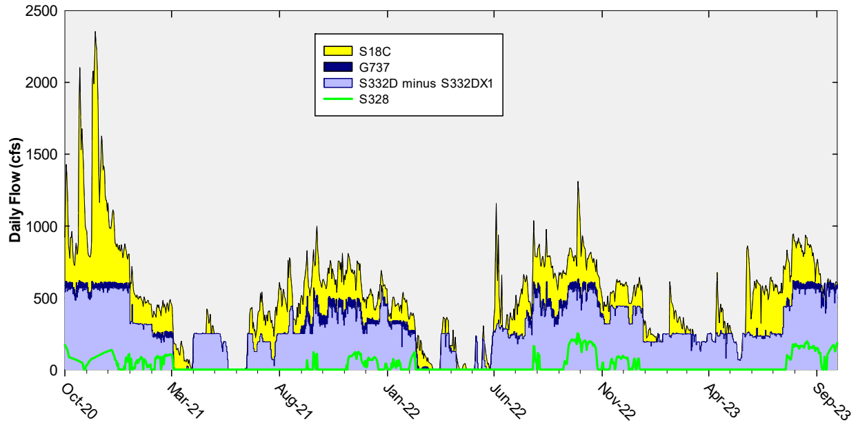
Figure 14. Daily flows into ENP as a stacked sum of Taylor Slough (G737 and S332D minus S332DX1) and Coastal Basins (S18C). S328 flow is shown as an overlaid line, and flow at this station downstream of S332D is associated with its own TP data.
