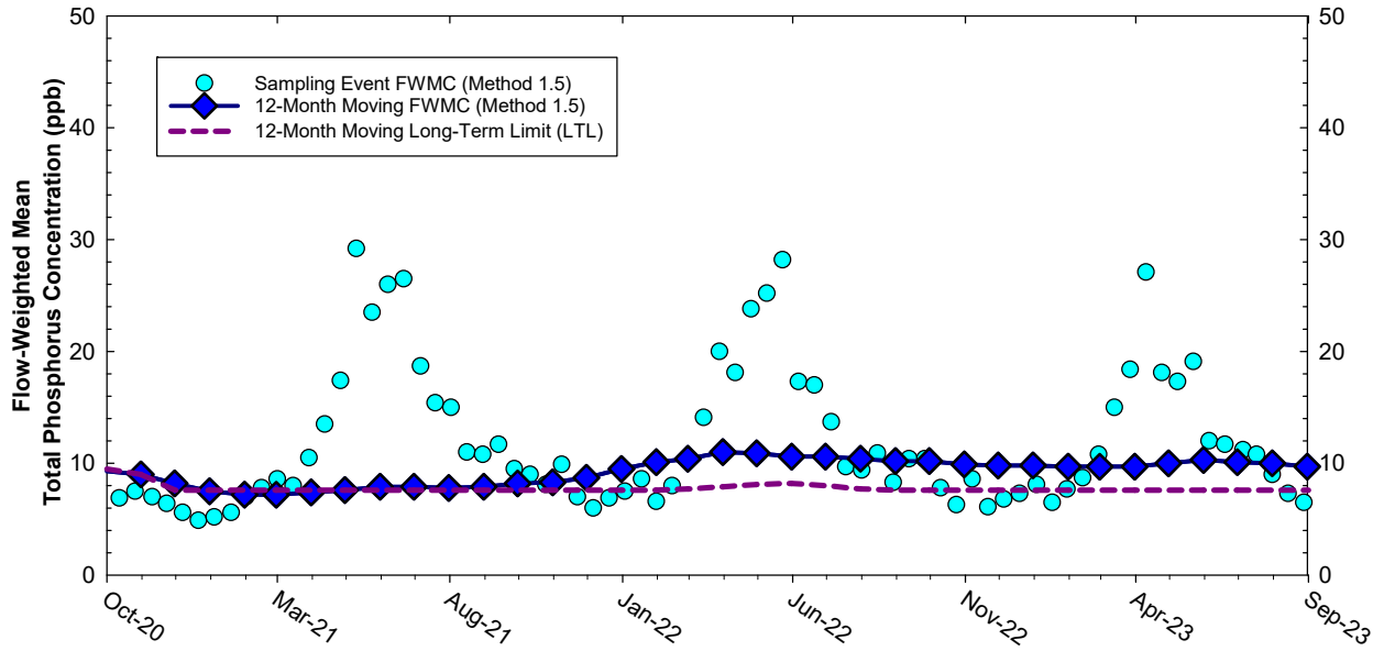
Figure 6. The 12-month TP FWMCs in inflows to ENP through Shark River Slough at the end of each month and TP FWMCs for each sampling event.
