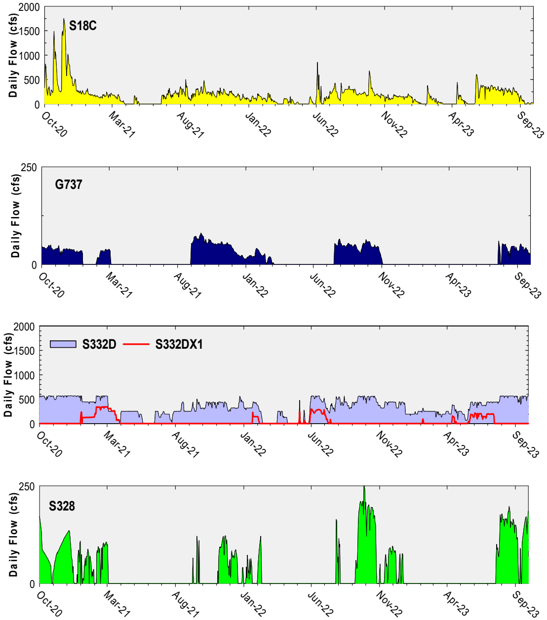
Figure 16. Daily flows in cubic feet per second (cfs) at individual Taylor Slough and Coastal Basins structures into ENP.
