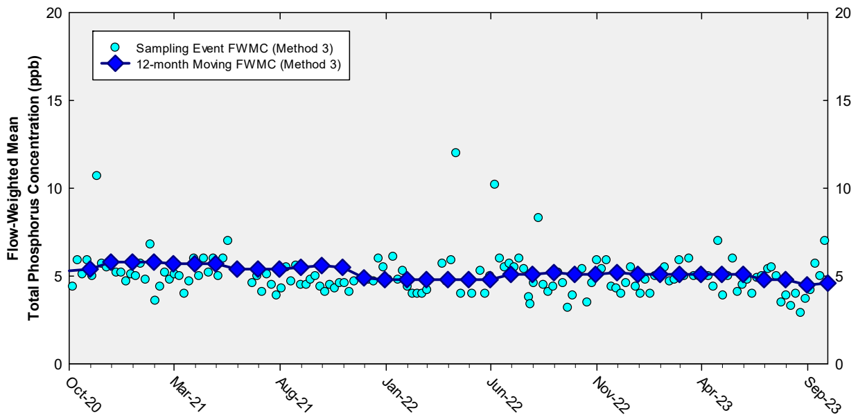
Figure 13. The 12-month TP FWMCs in inflows to ENP through Taylor Slough and Coastal Basins at the end of each month and the sampling TP FWMCs for each sampling event.
