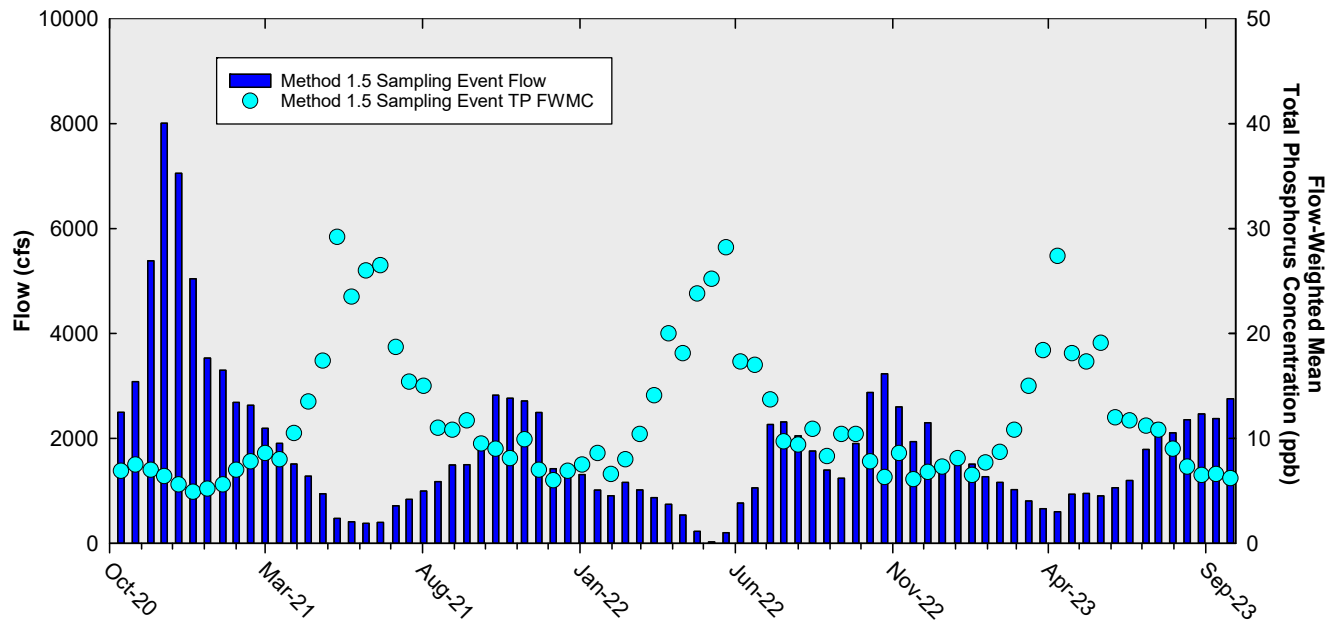
Figure 11. Flow to Shark River Slough on the day of sampling and the corresponding TP FWMCs for individual sampling events.
