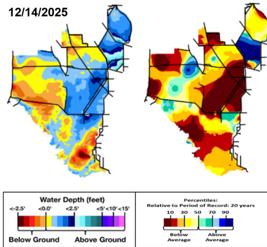
Figure EV-6. Present water depths (December 14, 2025) compared to the day of year relative to average (percentile) over the previous 20 years.
