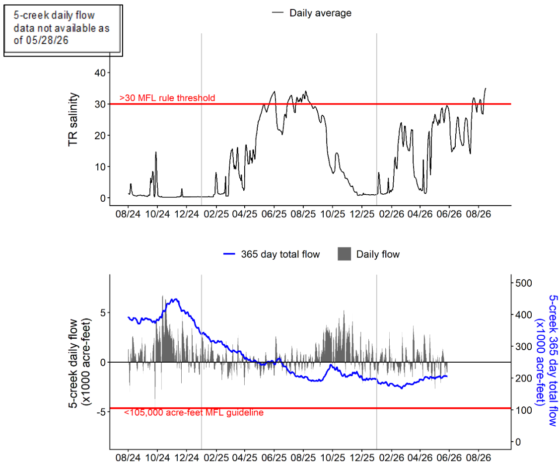
Figure EV-10. Daily average salinity at Taylor River (TR) tracked for the Florida Bay MFL criteria. The 365-day total creek flow MFL metric is not currently available due to missing creek flow data.
