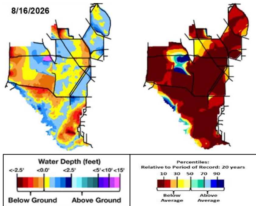
Figure EV-6. Present water depths (August 16, 2026) compared to the day of year relative to average (percentile) over the previous 20 years.
