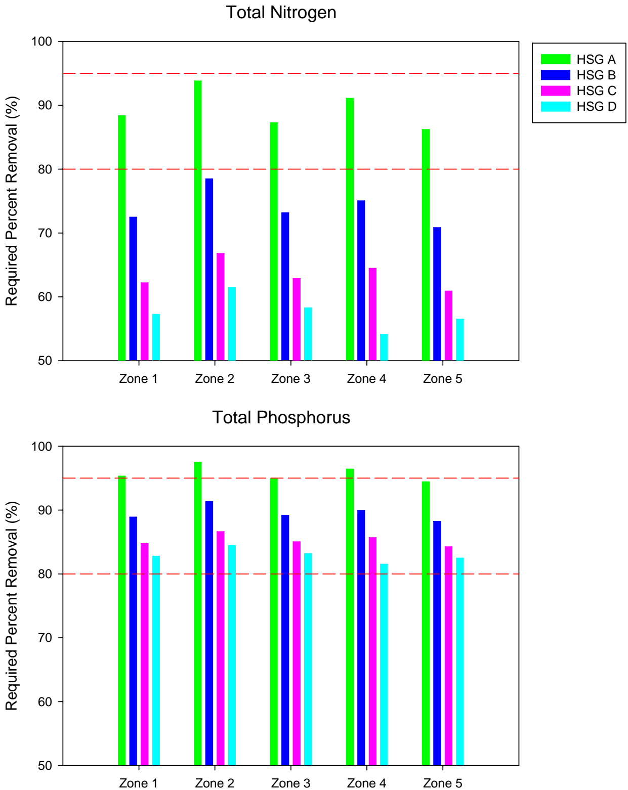
Figure 6-6. Comparison of Estimated Annual Mass Removal Efficiencies to Achieve Post-Development \leq Pre-Development Loadings of Nitrogen and Phosphorus for a Low-Density Residential Development.
