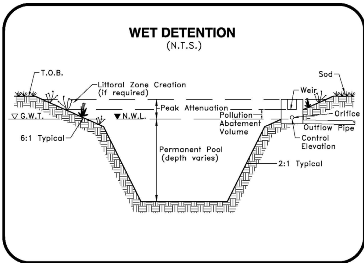
Figure 5-2. Schematic of a Wet Detention System.
