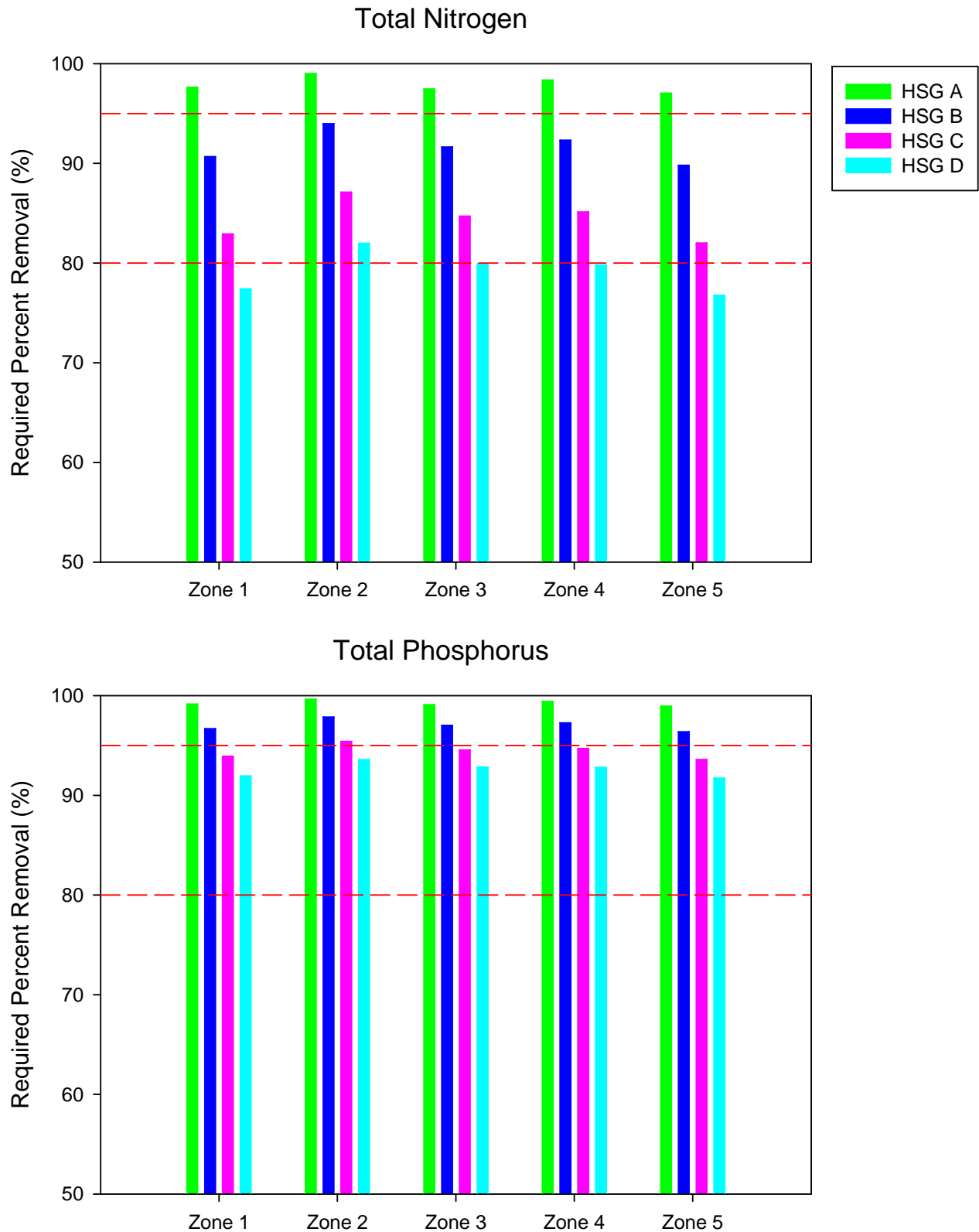
Figure 6-11. Comparison of Estimated Annual Mass Removal Efficiencies to Achieve Post-Development \leq Pre-Development Loadings of Nitrogen and Phosphorus for a Highway (50% Impervious) Development.
