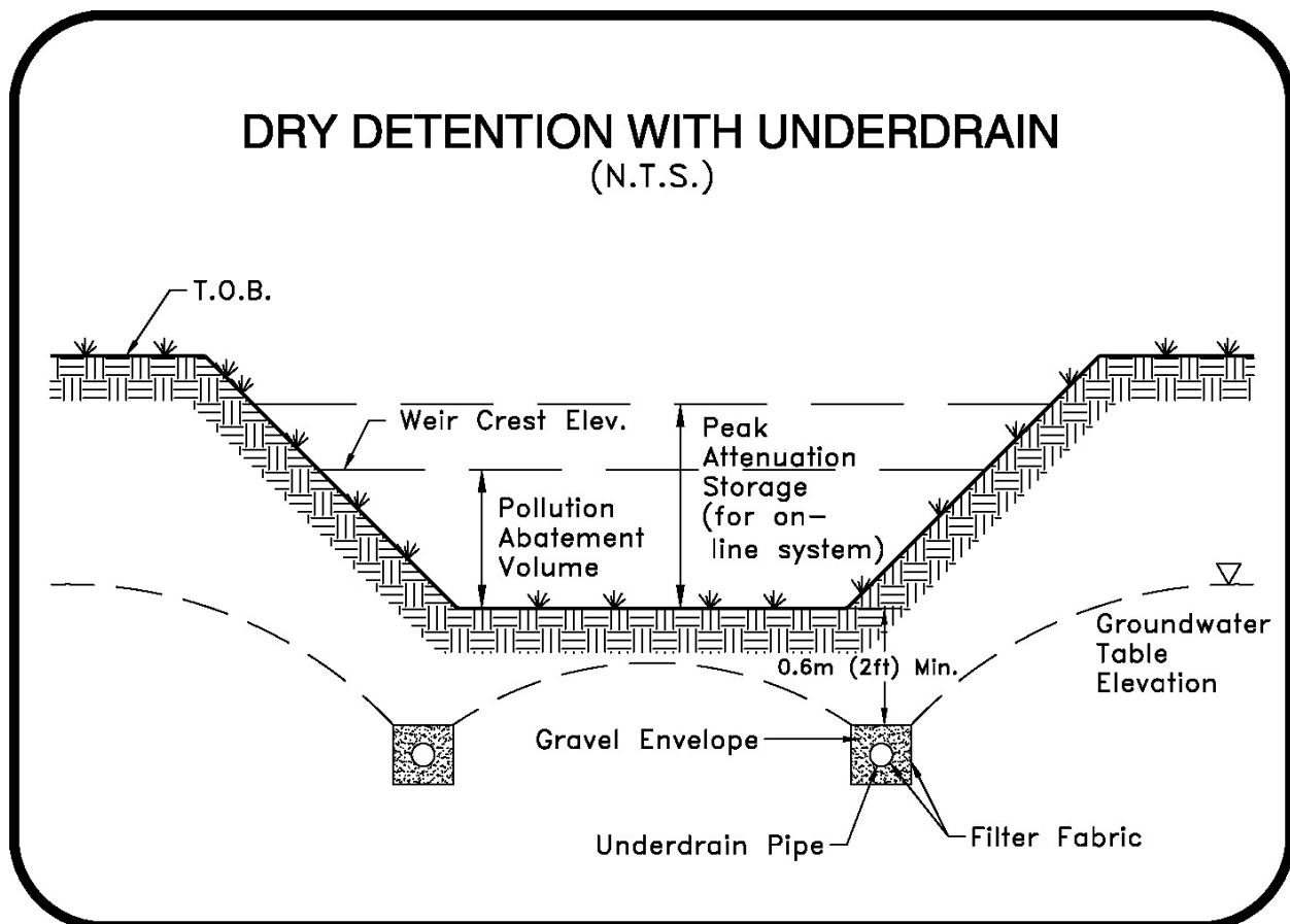
Figure 5-3. Schematic of a Dry Detention with Underdrain System.
