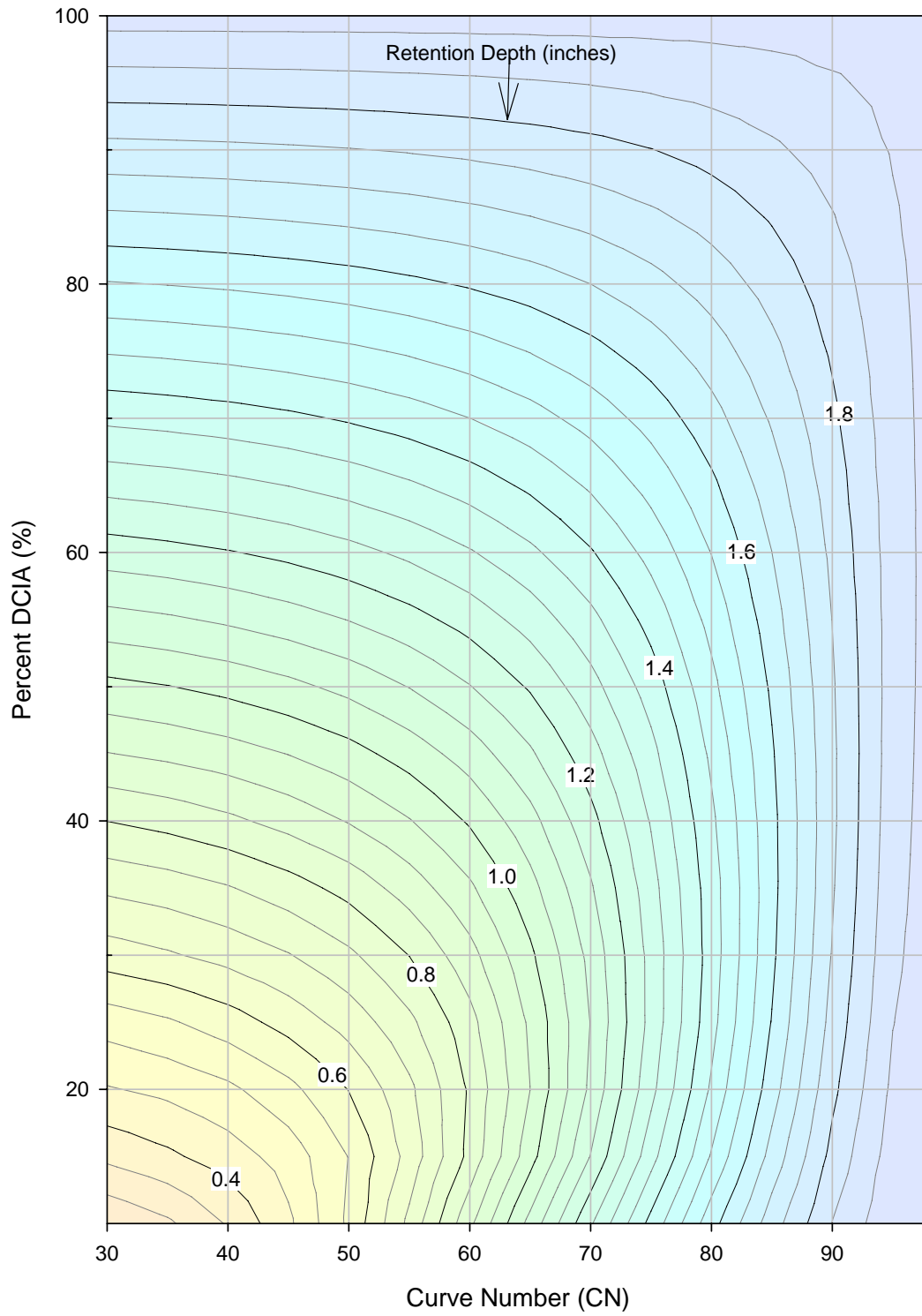
Figure 6-4. Variations in Required Dry Retention Depth to Achieve 80% Removal in the Panhandle Zone Area (Zone 1).
