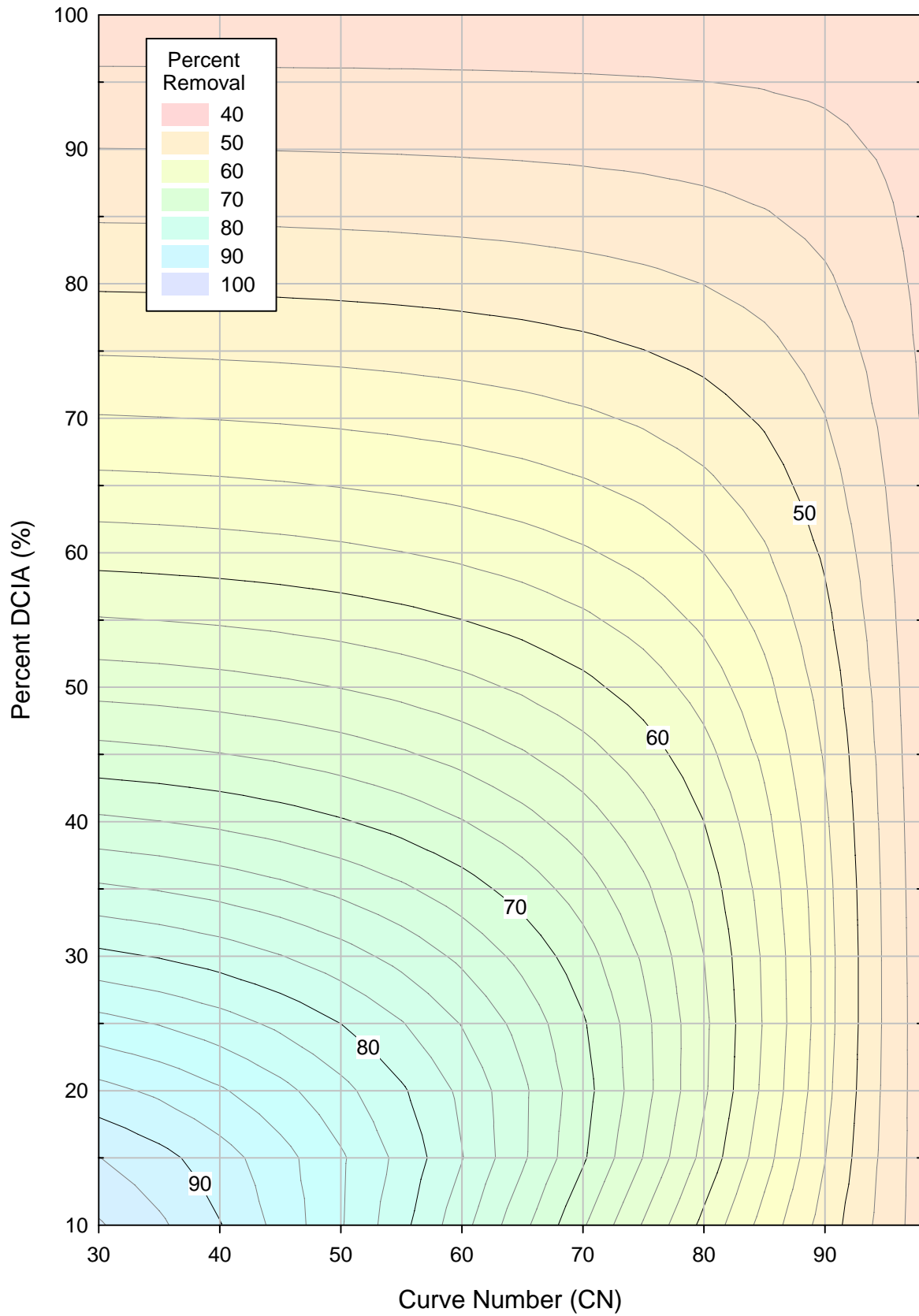
Figure 5-6. State-wide Average Removal Efficiencies for 0.5 inch of Dry Retention for Various DCIA Percentages and non-DCIA Curve Numbers.
