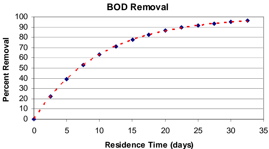
Figure 6-1. Theoretical Removal of BOD as a Function of Residence Time in a Wet Detention Pond.
