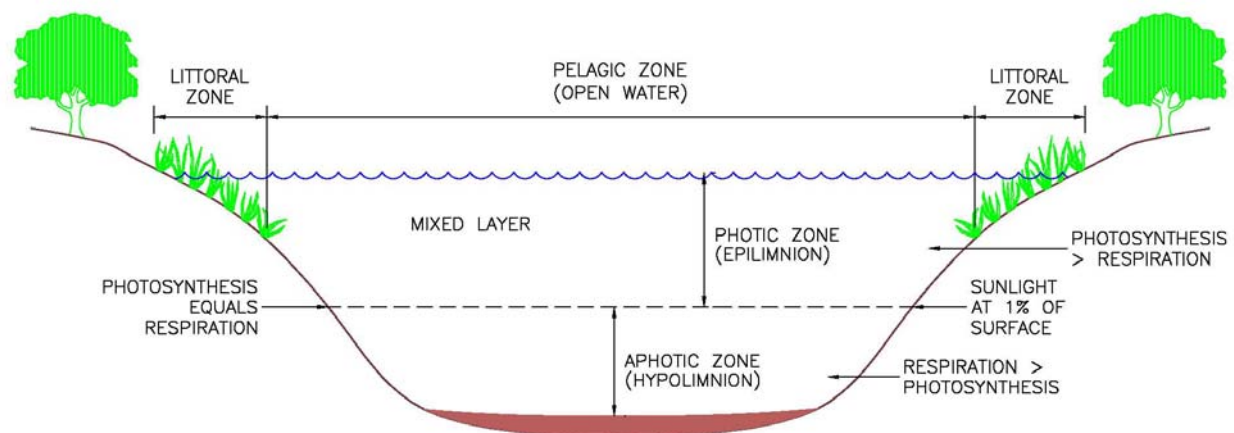
Figure 6-13. Typical Zonation in a Lake or Pond.
