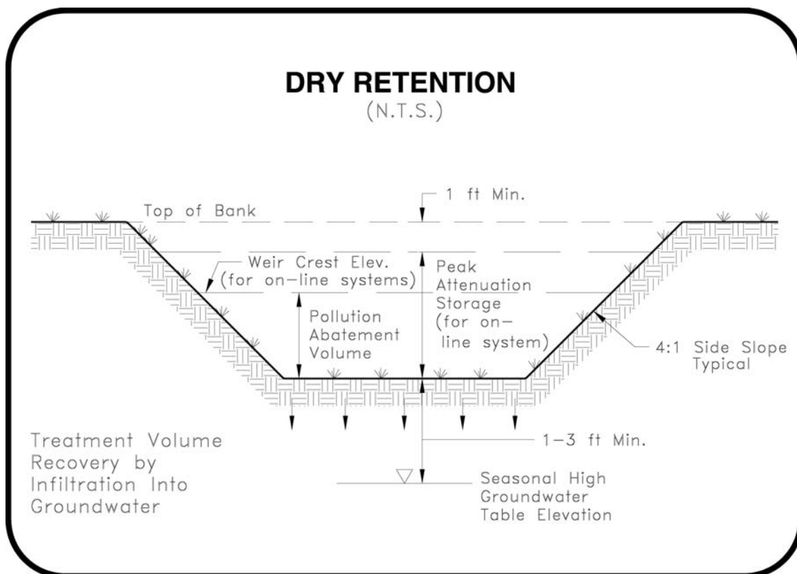
Figure 5-1. Schematic of a Dry Retention Facility.
