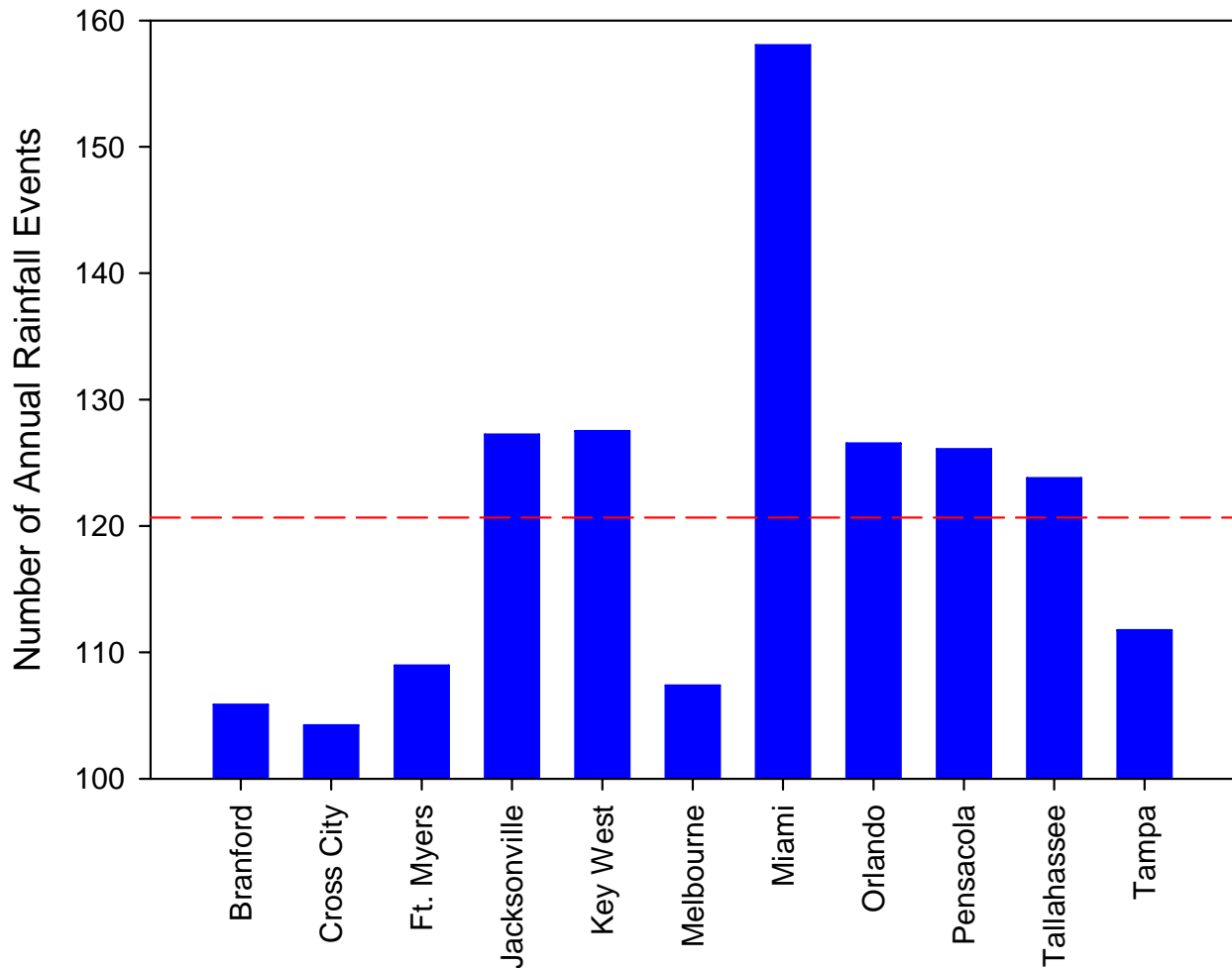
Figure 3-5. Comparison of the Mean Number of Annual Rainfall Events at the Selected Regional Sites.
