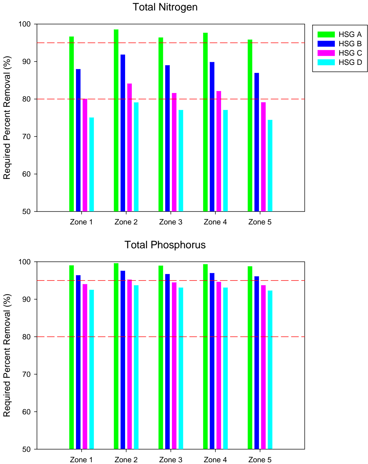
Figure 6-8. Comparison of Estimated Annual Mass Removal Efficiencies to Achieve Post-Development \leq Pre-Development Loadings of Nitrogen and Phosphorus for a Single-Family (40% Impervious) Residential Development.
