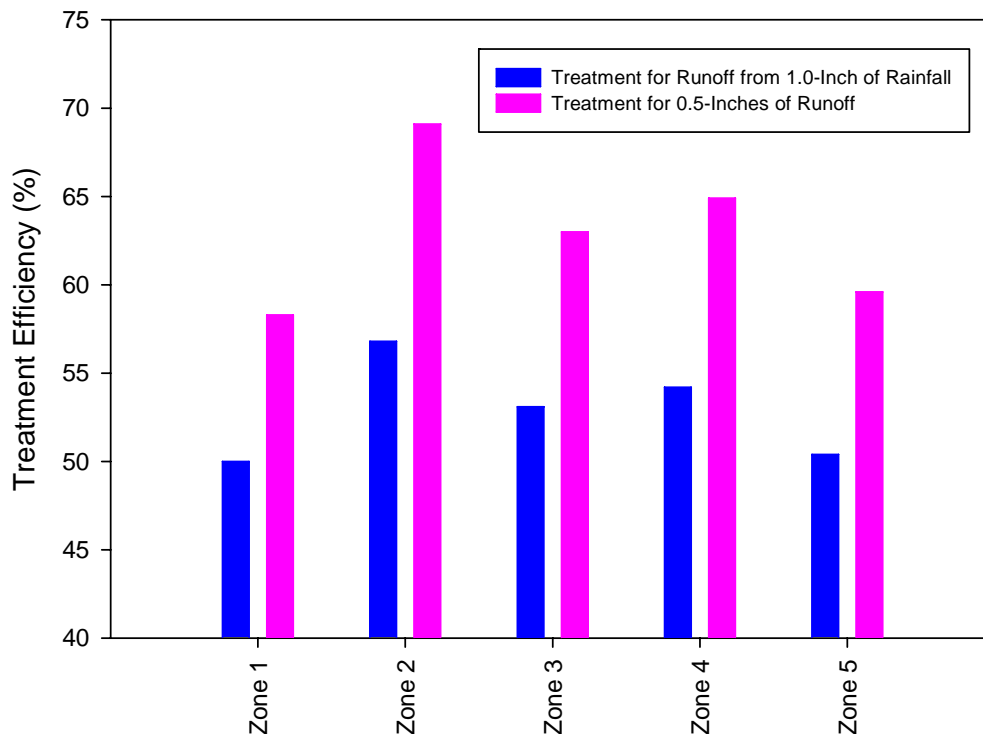
Figure 5-8. Comparison of Annual Mass Removal Efficiencies for Dry Retention Systems Designed for Treatment of 0.5 inch of Runoff or the Runoff from 1 inch of Rainfall.
