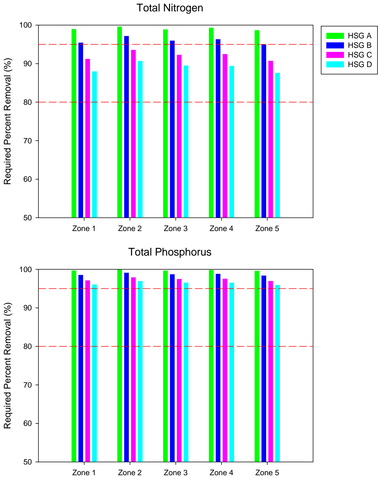
Figure 6-10. Comparison of Estimated Annual Mass Removal Efficiencies to Achieve Post-Development \leq Pre-Development Loadings of Nitrogen and Phosphorus for a Commercial Development.
