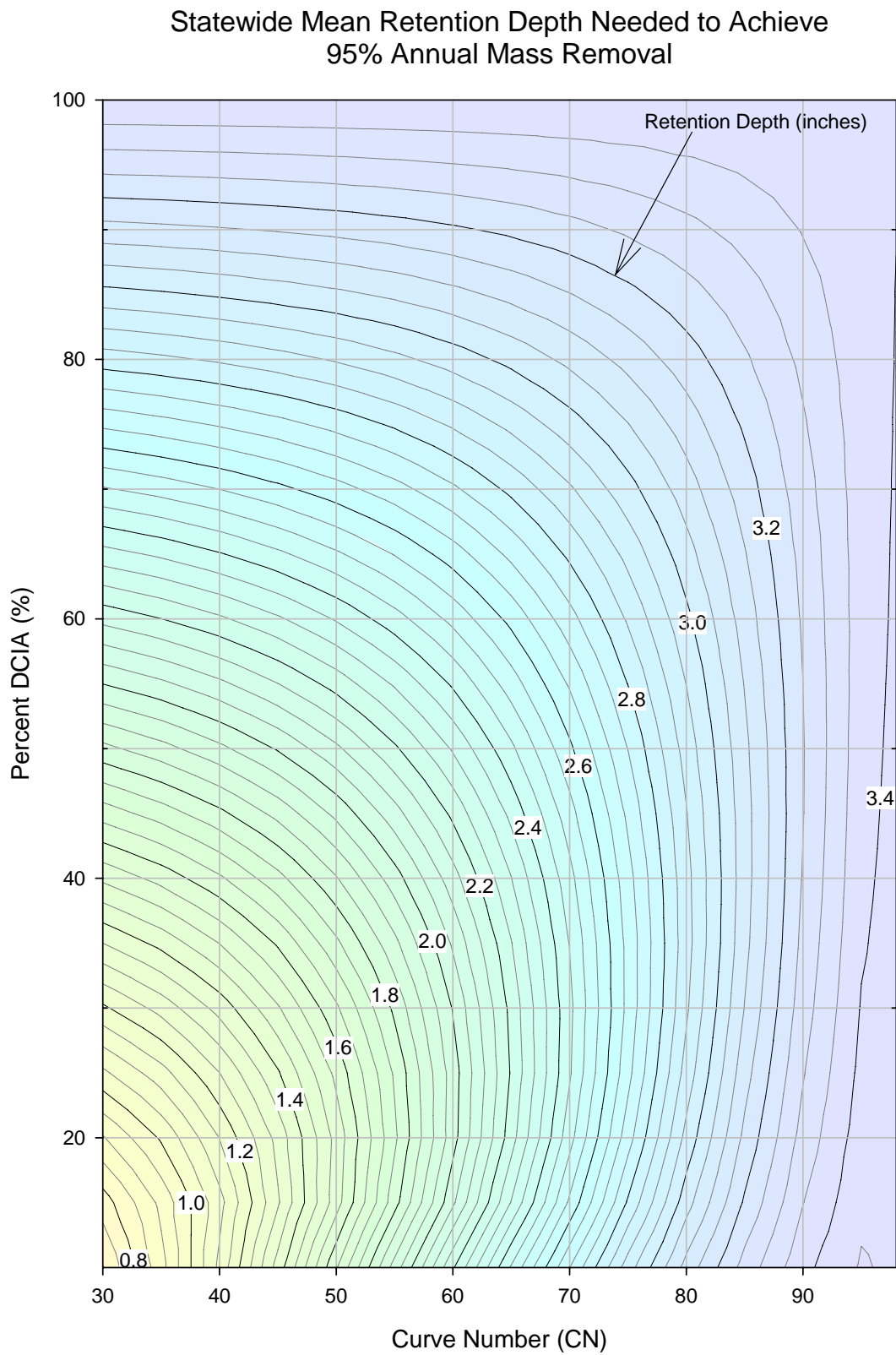
Figure 6-5. Variations in Required Dry Retention Depth to Achieve 95% Removal on a State-wide Basis.
