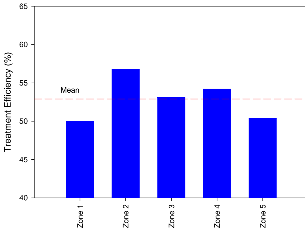
Figure 5-7. Calculated Annual Mass Removal Efficiencies for Dry Retention of the Runoff from 1 inch of Rainfall for a Development with 40% DCIA and a non-DCIA Curve Number of 70.
